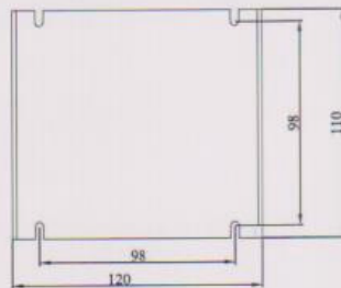
CONTROLLER
